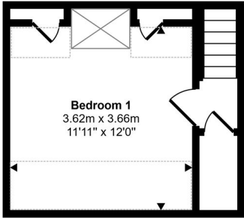
Second Floor Approx 18 sq m / 196 sq ft
