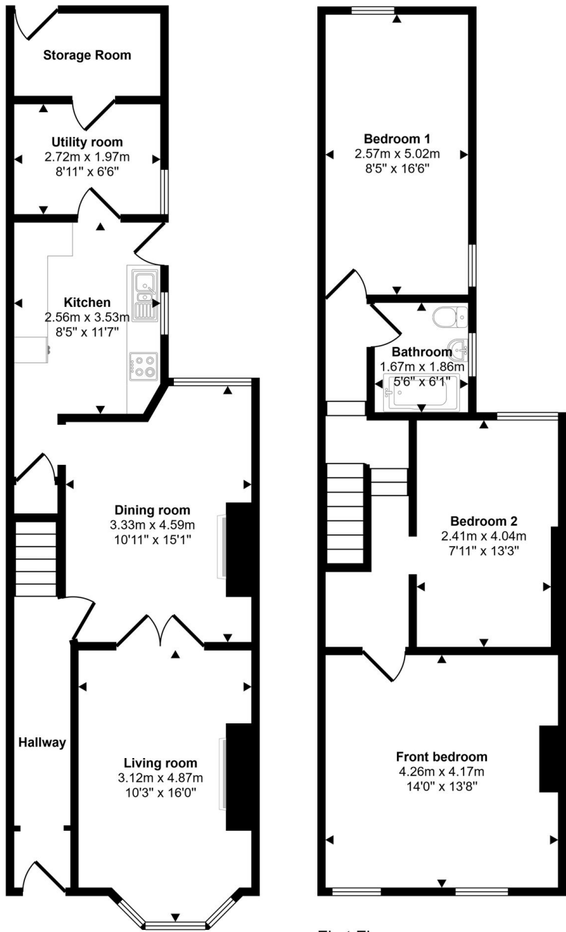
First Floor Approx 54 sq m / 582 sq ft
